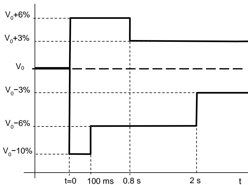
Figure 6 — Voltage characteristic for infrequent events
